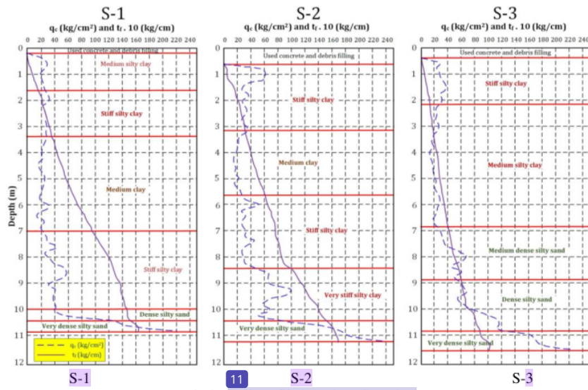
Fig.2a Soil profile based on CPT data
