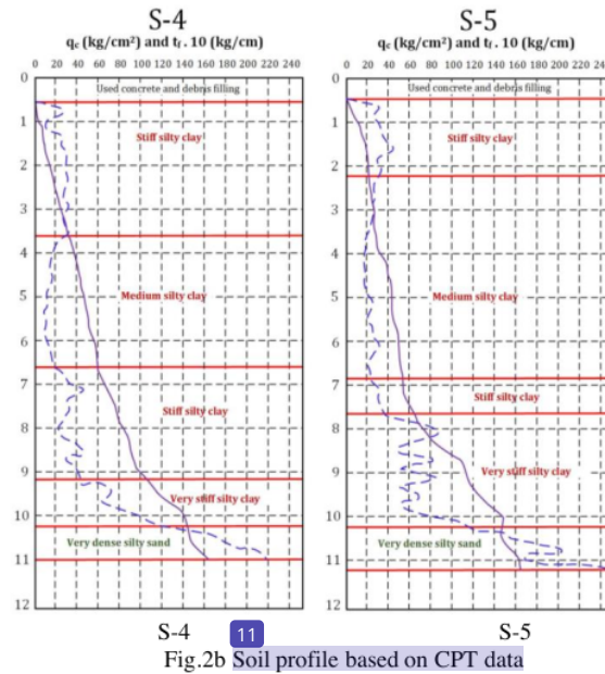
Fig.2b Soil profile based on CPT data
