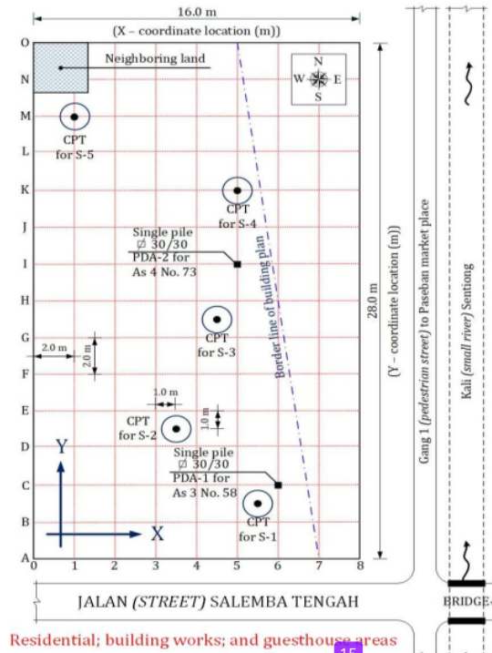
Fig. 1 Layout of CPT and PDA tests in the study area
