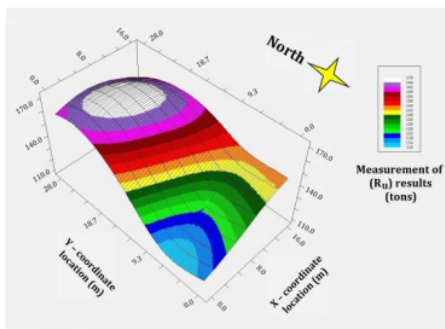
Fig. 7 Measurement results of R_u (PDA)
