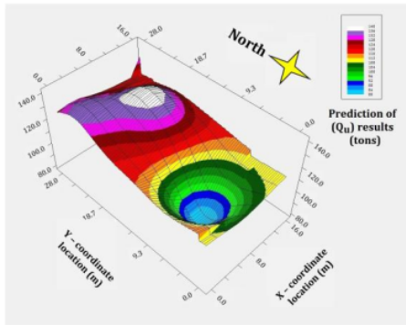
Fig. 6 Prediction results of Q_u (CPT)
