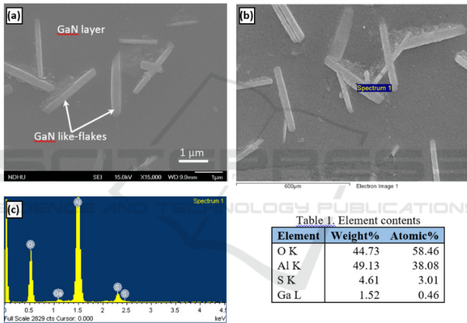
Figure 3. SEM images of surface morphology GaN layers (a, b), and (c) EDS of scan-spot on the surface GaN like-flakes
