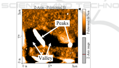
Figure 1. AFM image of 2D MoS 2 layer deposited on the sapphire substrate
