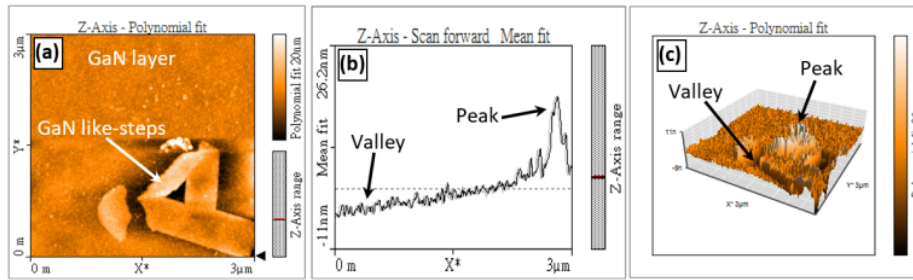
Figure 2. AFM images of surface GaN layer observed; (a) Scan area profile of 3x3 \mu\text{m} , (b) line-profile through of 3 \mu\text{m} , and (c) 3-dimension profile with a deep of 20 nm
