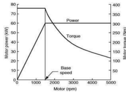
Figure 2. Types of electric motor characters [17]
