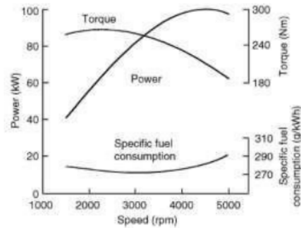
Figure 1. Types of gas engine characters [17] Internal combustion engines have a relatively flat (compared to ideal) torsion speed profile, as shown in Figure 1.
