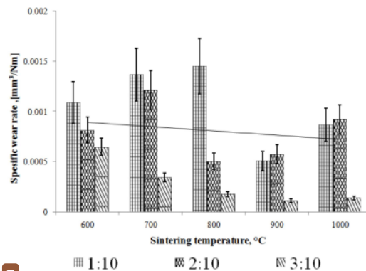
Fig. 10. The relationship of specific wear rate vs. sintering temperature.
