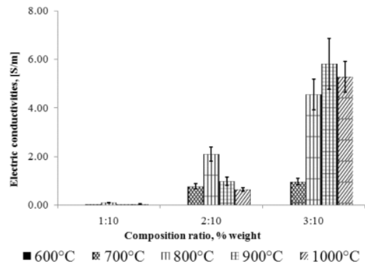
Fig. 6. The relationship of electrical conductivity vs. composition ratio.
