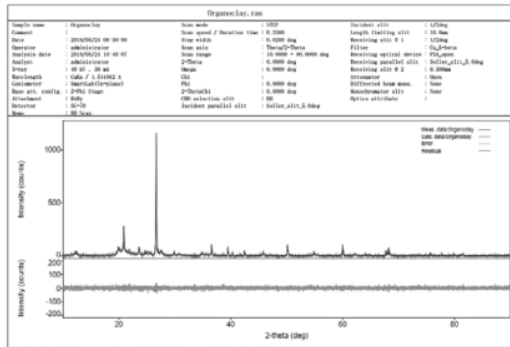
Fig. 1. X-Ray powder Diffractogram of organoclay.
