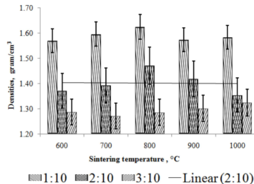
Fig. 12. The trend of the densities of carbon ceramic composites.
