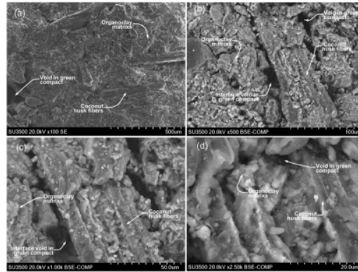
Fig. 3. Morphology of composite green compact (before sintering).
