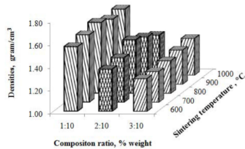
Fig. 11. The densities vs composition ratio vs sintering temperature.
