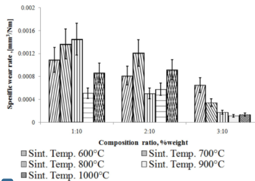
Fig. 9. The relationship of specific wear rate vs. composition ratio.
