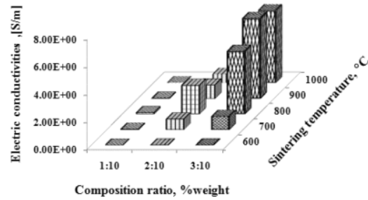
Fig. 5. The electrical conductivity of carbon ceramic composite.
