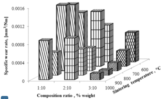
Fig. 8. The relationship of specific wear rate vs. composition ratio vs. sintering temperature.
