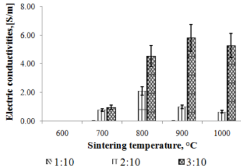
Fig. 7. The relationship of electrical conductivity vs. sintering temperature.
