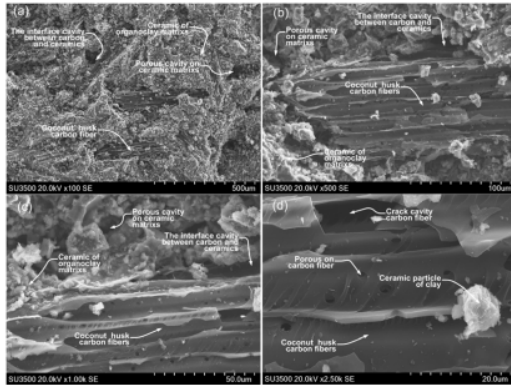
Fig. 4. Morphology of carbon ceramic composite.
