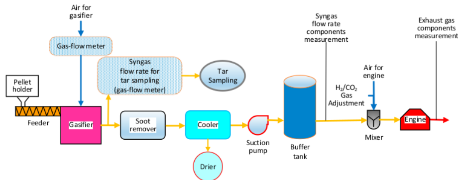
Figure 1. The biomass gasification system.
