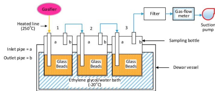
Figure 2. Tar-Sampling Equipment.
