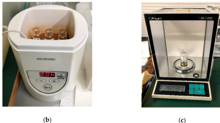
Figure 3. (a) Shimadzu GC-MS QP2010 Plus (b) Dryer–evaporation machine (IRIS OHYAMA) (c) Tar-weight measurement machine (Chyo JL-200).
