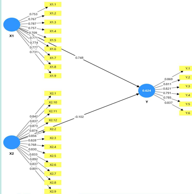
Outer loadings - Matrix
