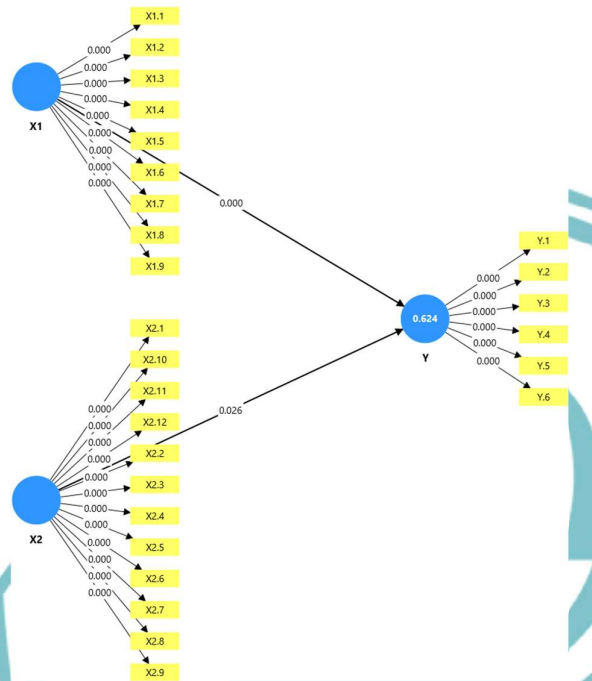
Path coefficients - Mean, STDEV, T values, p values
