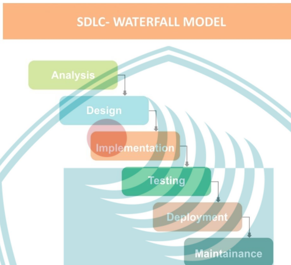
Gambar 1.1 Metode WATERFALL
