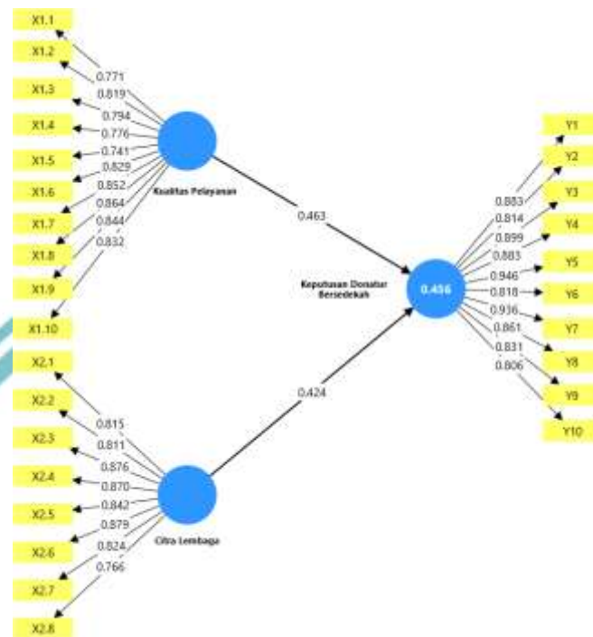
Outer loadings - Matrix
