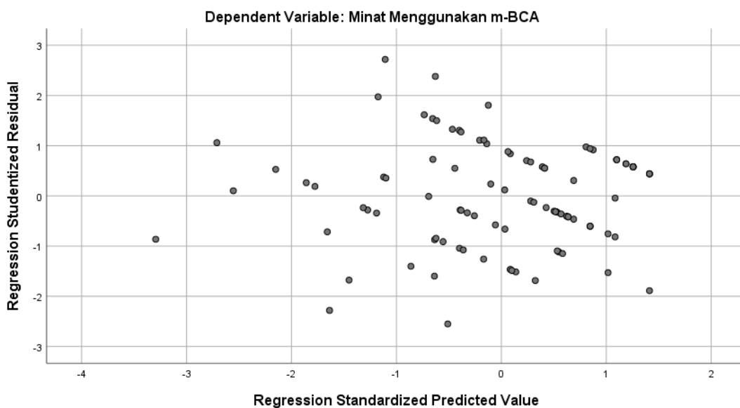
Scatterplot
