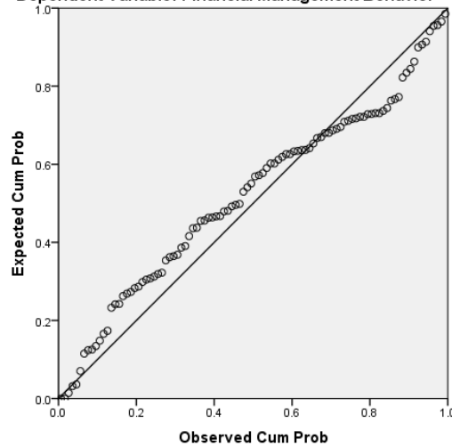
Normal P-P Plot of Regression Standardized Residual Dependent Variable: Financial Management Behavior
