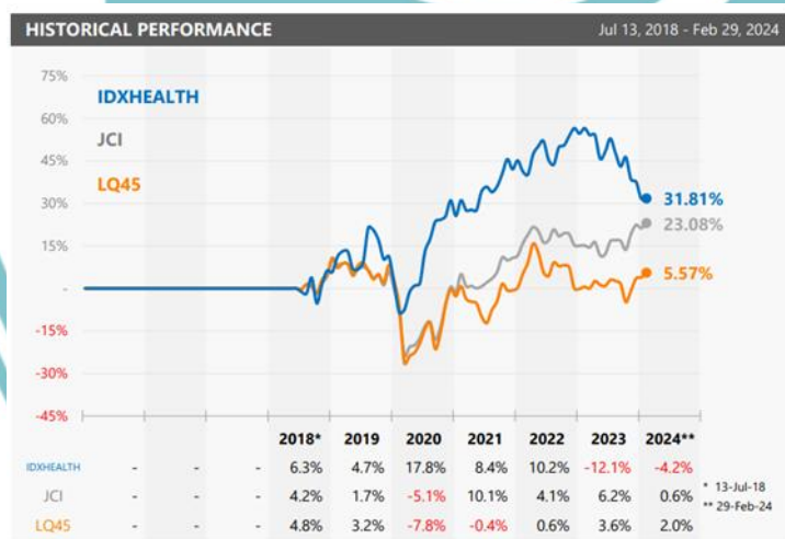
Gambar 1. 1 Historical Performance IDXHEALTH
