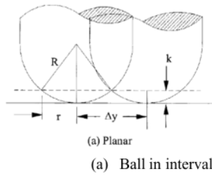
Figure 7 Ball-End Mill Cutting Interval (Yau & Hsu, 2009)
