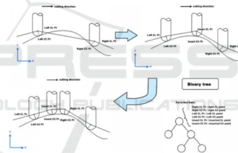
Figure 10 Ball-End Mill Overcut Condition and the Solving by Using Buffer Point (Yau & Hsu, 2009).
