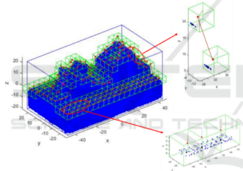
Figure 8 Ball-End Mill Path Checking
