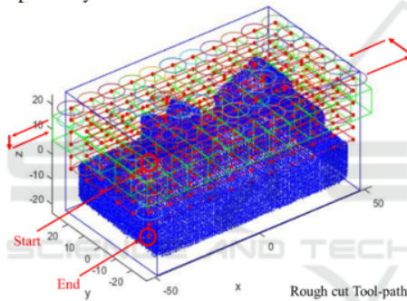
Figure 12 Rough Cutting CL Computation Result
