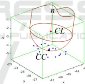
Figure 6 Ball-End Mill Position
