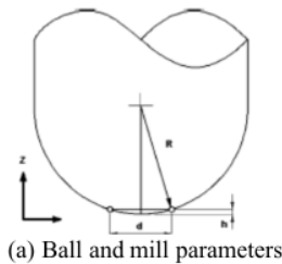
Figure 6 Ball-End Mill Position
