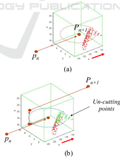
Figure 3 Evaluation of Next Step of Tools (a) CC Cut Point Cloud (Over-Cut) and (b) the Solution by Moving CC of the Tools
