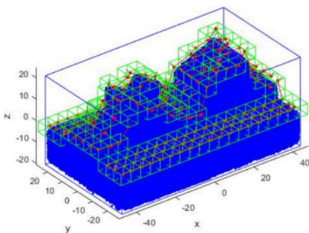
Figure 13 Semi-finished Cutting CL Computation Result
