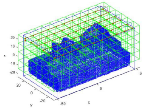
Figure 1 Grid System for Rough Cutting by Using Flat-End Mill
