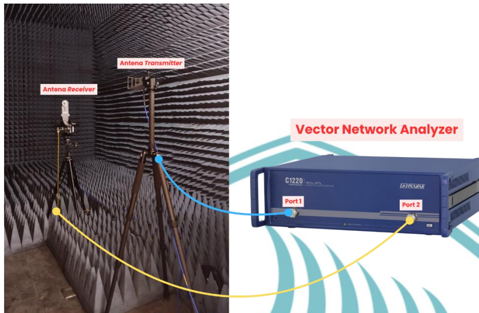
Gambar 4.2 Set Up Pengujian Dual Port
