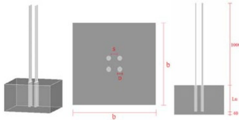
Fig. 4. Specimen Details
