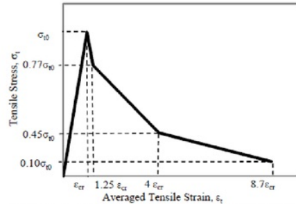
Fig. 3 Tension Stiffening Modeling at ABAQUS Manual (2008)
