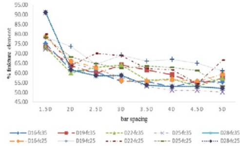
Fig. 6. Damage Percentage of Grouting to Reinforcement Distances
