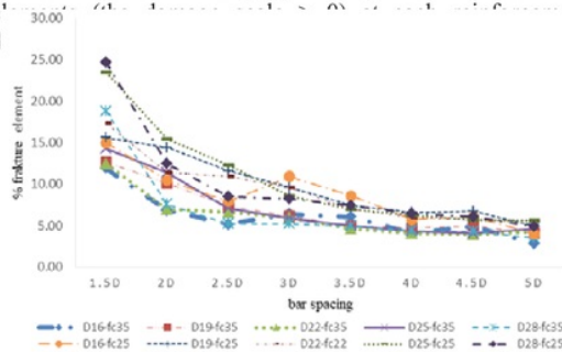
Fig. 5. Damage Percentage of Concrete to Reinforcement Distances
