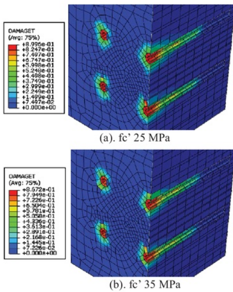
Fig. 16. Visualization of Parameter on Failure Tensile on Specimens D28-4D: (a) f_c' 25 MPa, (b) f_c' 35 MPa
