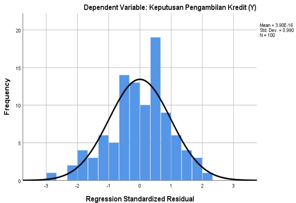
Histogram
