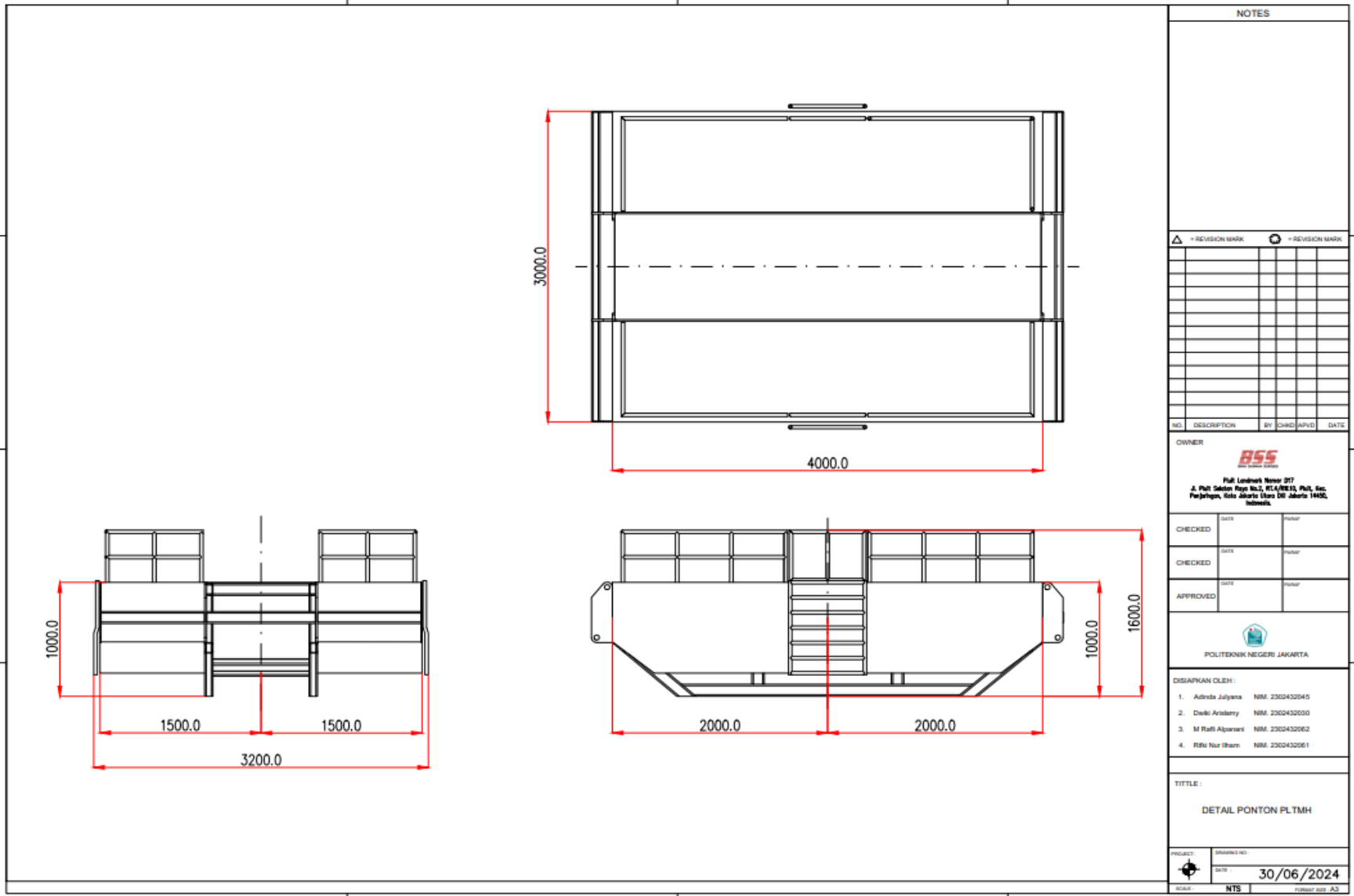
Lampiran 5. Design & Ukuran Ponton JAKARTA
