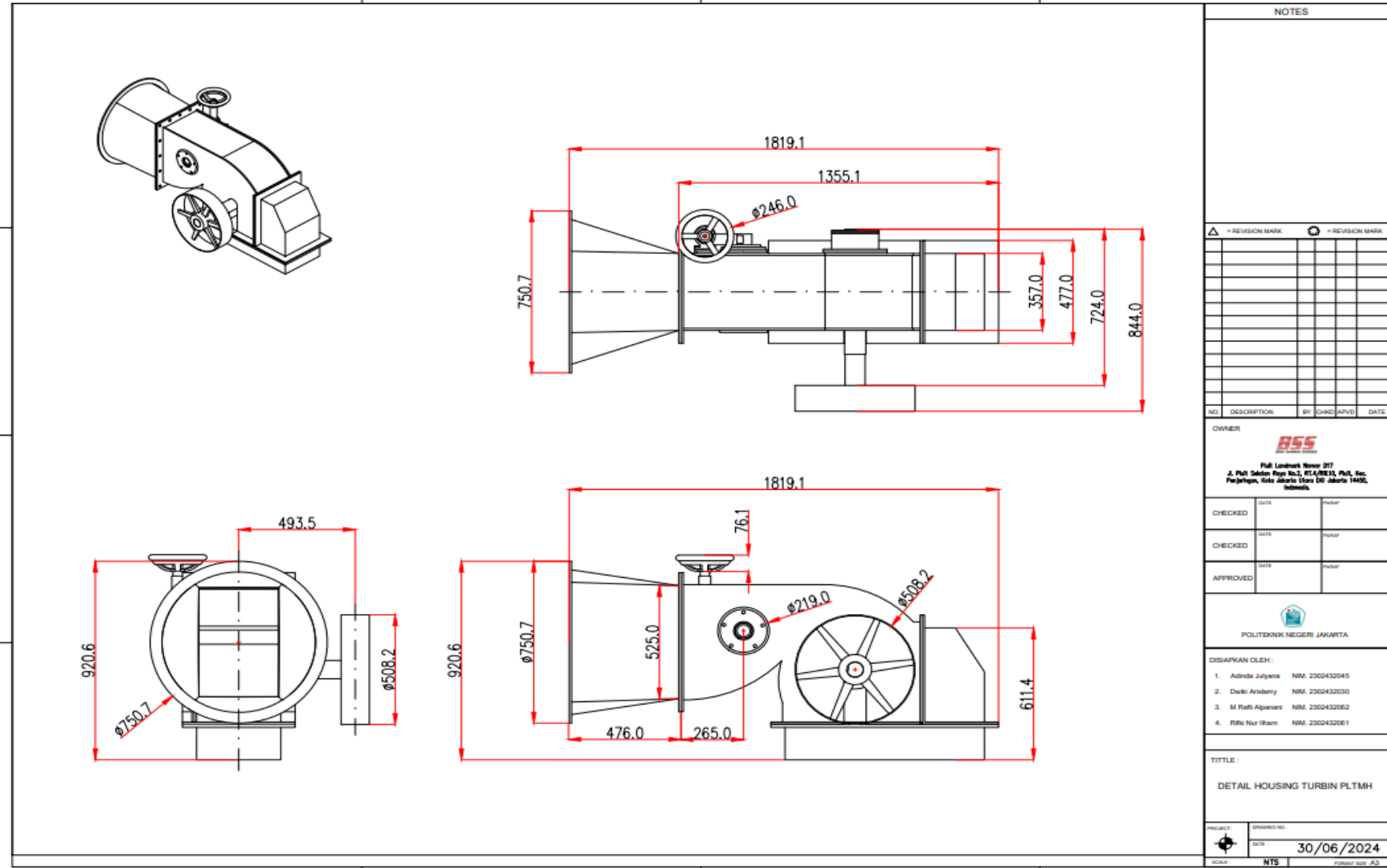
Lampiran 6. Design & Ukuran Turbin Crossflow
